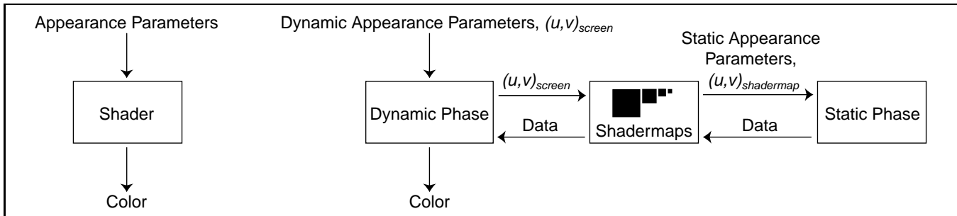
Figure 1: Dataflow diagrams for a traditional shader and a shader using shadermaps. On the right, the shader has been separated into its dynamic and static phases. The shadermap is similar to a cache between the two phases. Though not shown, the (u, v)_{screen} and dynamic appearance parameters include screen-space derivatives, necessary for the anisotropic filter. The (u, v)_{shadermap} and static appearance parameters include (u, v) space derivatives, used for antialiasing.
