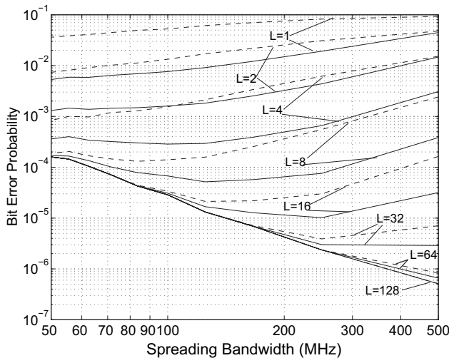
Fig. 6. The BEP vs. the spreading bandwidth in a Log-Log scale for different numbers of PRake (dashed) and SRake (solid) fingers in the Nakagami LF model. The Tx-Rx distance is 6 m and the average transmitted SNR is 30 dB.
