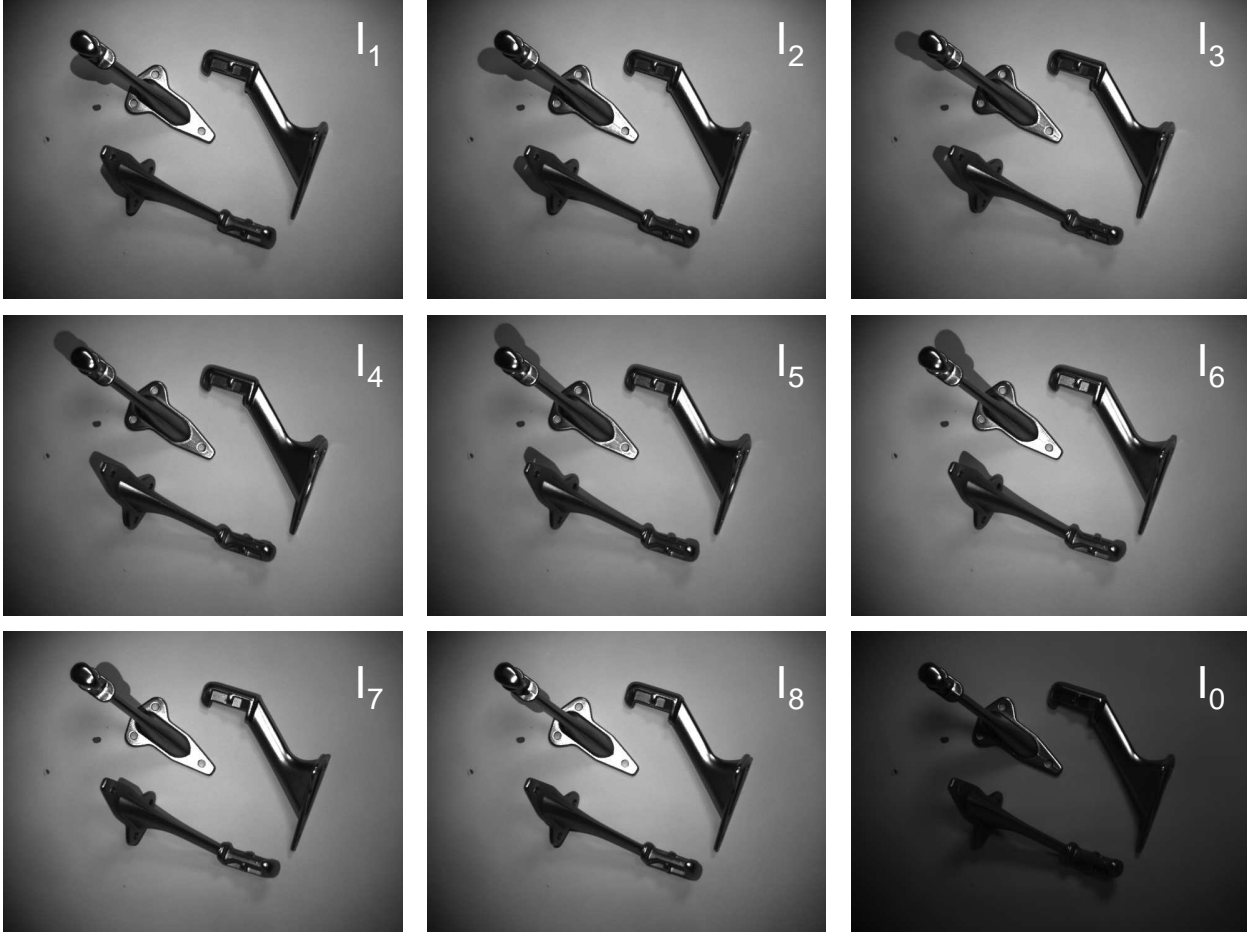
Figure 4: Captured images of a scene with three brass hooks using our camera. I_1 to I_8 correspond to the images taken with different flashes ( I_1 corresponds to the image taken with the flash on top of the camera). I_0 corresponds to the image taken without any flash. Notice how the shadows move with the position of the flash.
