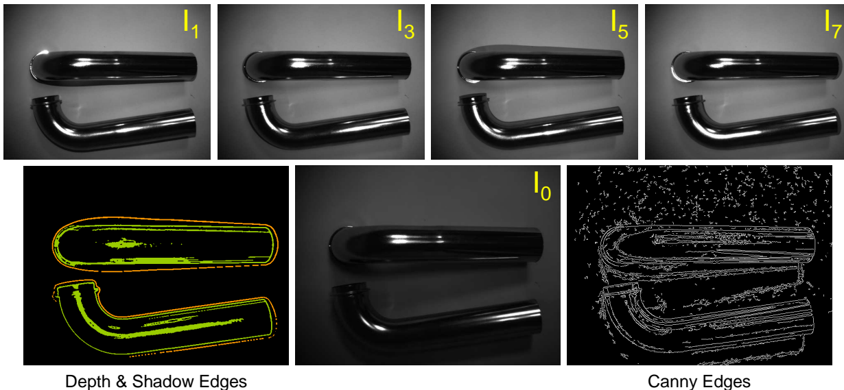
Figure 16: Specular objects. 3D range scanners does not provide reliable geometry information on specular objects. In addition, reliable 2D intensity based features are not also not obtained on specular objects due to inter-reflections. Our approach can easily handle specular objects and estimate reliable depth edges.
