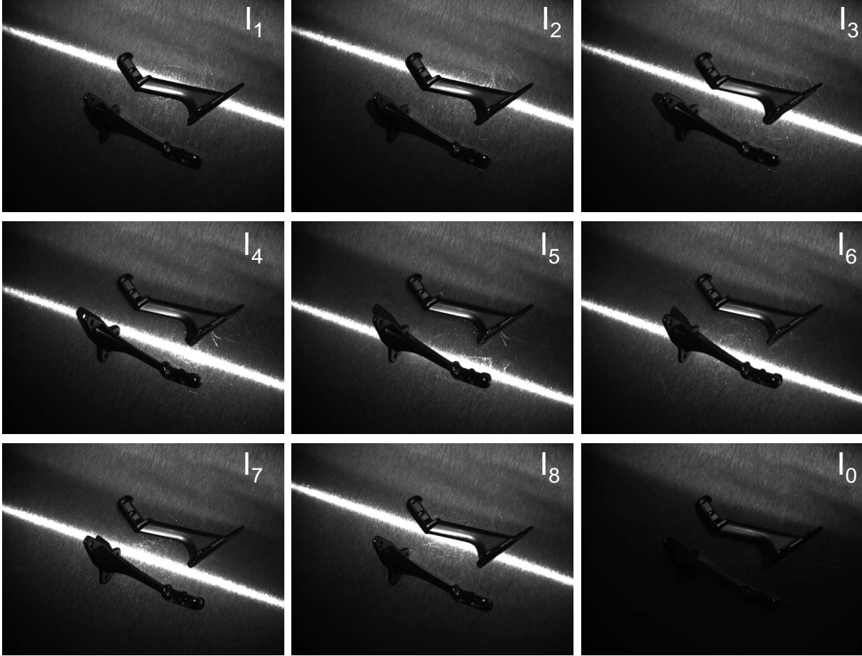
Figure 11: Non-uniform shiny background. A metallic plate is placed as the background. The ambient illumination image I_0 shows non-uniform illumination on the background. Captured images with flash shows specularities and highlights due to the metallic plate. These can be removed if their location in the image changes.
