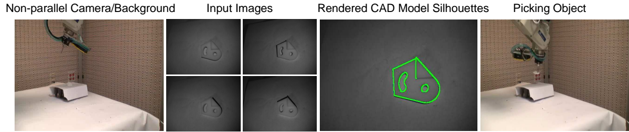
Figure 18: Generality of the proposed method. The image plane of the camera does not have to be parallel to the background, and objects can have holes.
