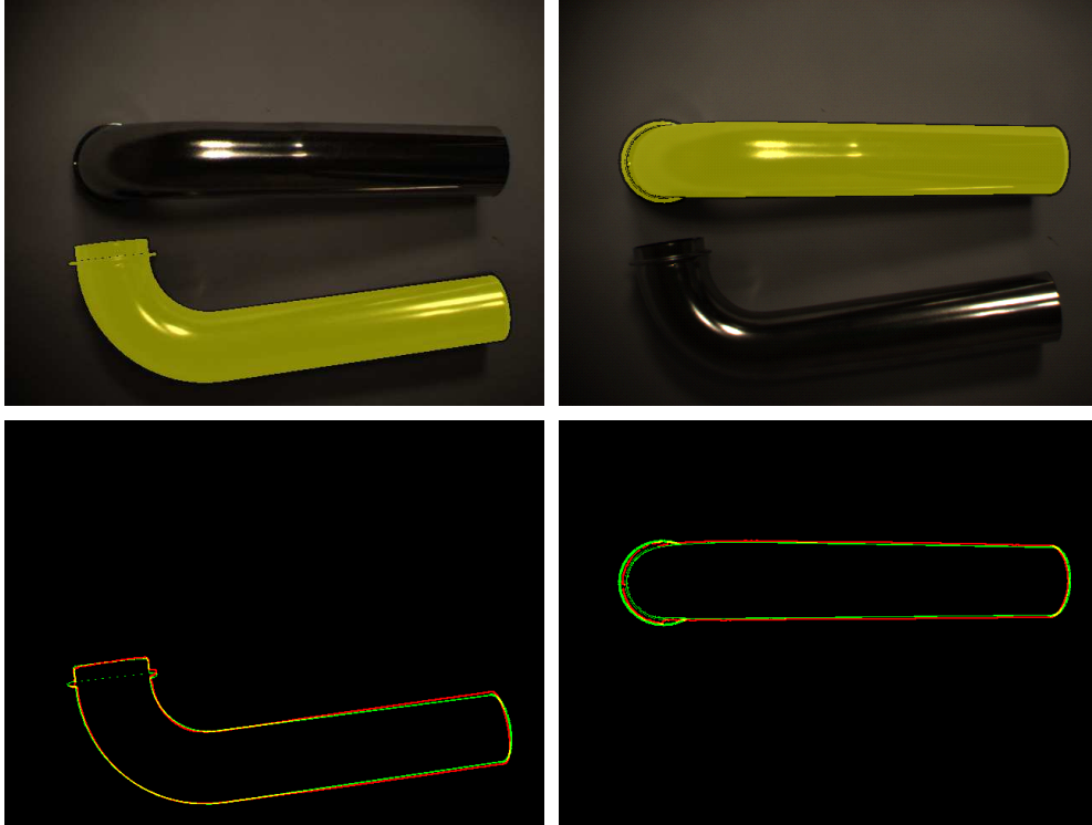
Figure 17: Pose estimation results on objects shown in Figure 16. Top row shows the overlay of the rendered CAD model on I_0 and the bottom row shows the overlay of the rendered CAD model silhouette on the segmented object silhouette according to the final estimated pose for both objects.
