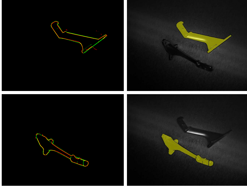
Figure 13: Non-uniform shiny background. Overlay of the rendered CAD model silhouette on the segmented object silhouette and the rendered CAD model on I_0 for both objects after fine pose estimation. Note that although depth edges have noise, silhouettes used for pose estimation are clean as only the outermost object boundary is utilized.
