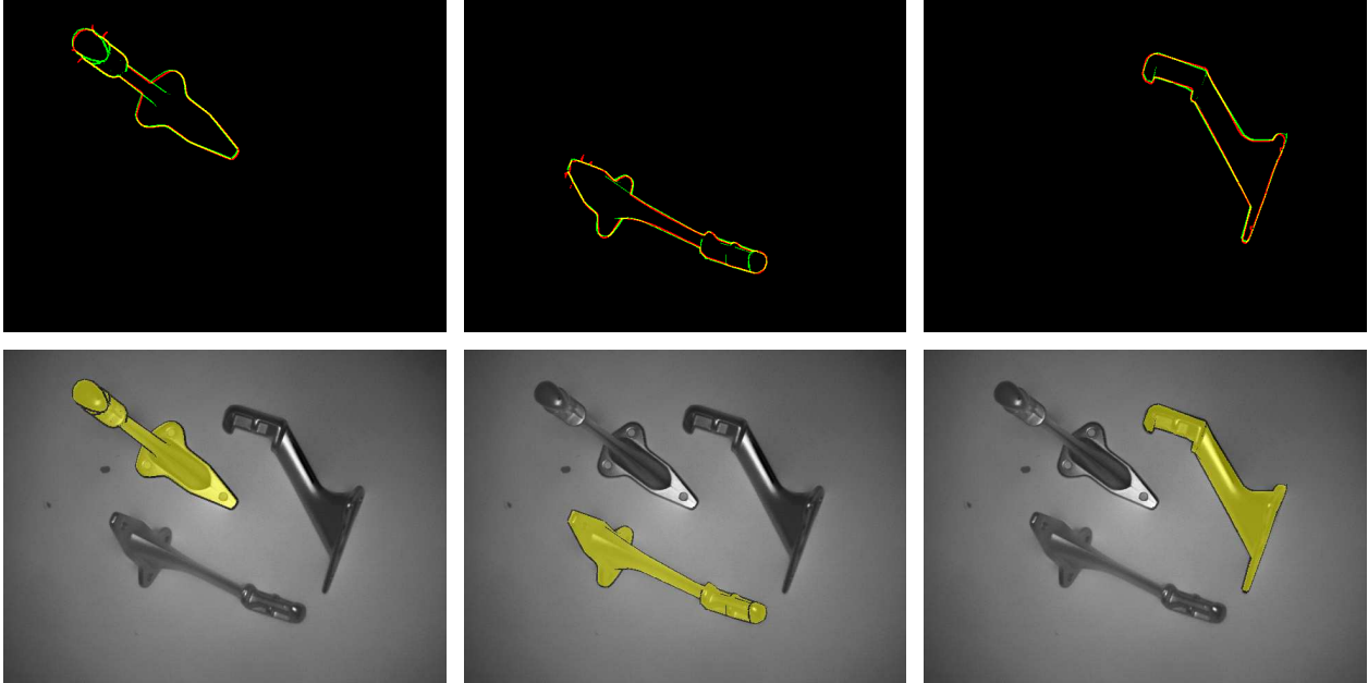
Figure 10: 3D pose estimation results for all three objects shown in Figure 4. Top row shows the overlay of the rendered CAD model silhouette (green) according to the final estimated pose on the segmented object silhouette (red). Bottom row shows the overlay of the rendered CAD model according to the final estimated pose on I_0 .
