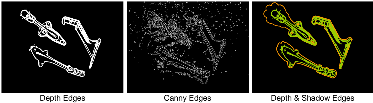
Figure 6: Detected depth edges (green) and shadow edges (orange) using our approach on the scene shown in Figure 4. In comparison, Canny edges [Can86] on ambient image I_0 are also shown in the middle. Note that the Canny intensity edges are noisy and do not provide reliable features due to the non-Lambertian reflectance properties of the brass hook.
