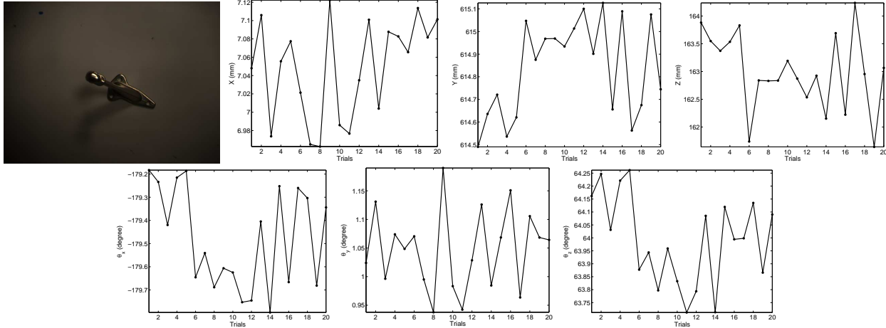
Figure 21: Repeatability analysis for pose estimation: The pose of the brass hook as shown was estimated 20 times from the same camera position. Shown are the plots for the estimated translation and rotation angles of the pick point. The true location and pick angles was determined manually using teach-box to be X = 7.9 mm, Y = 612.62 mm, Z = 164.68 mm, \theta_x = -180^\circ , \theta_y = 0^\circ and \theta_z = 65.33^\circ .
