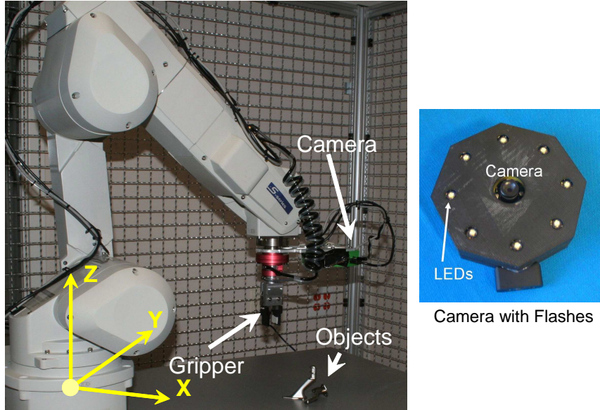
Figure 1: Experimental setup. A six degree of freedom (DOF) robot arm equipped with a pneumatic gripper is used for experiments. The camera attached to the robot arm is housed inside a plastic case and is surrounded by eight light emitting diodes (LED's) controlled by a micro-controller. Objects to be picked are placed on a table as shown. The world coordinate system is attached to the base of the robot with the axis directions as shown.
