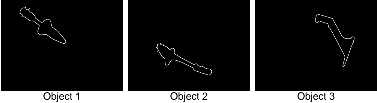
Figure 8: Segmentation of depth edges into different objects. Depth edges inside the object (internal silhouettes) are ignored to avoid spurious edges due to specular reflections and only external silhouettes are kept. Each of these three silhouettes is used to estimate the pose of the corresponding object.
