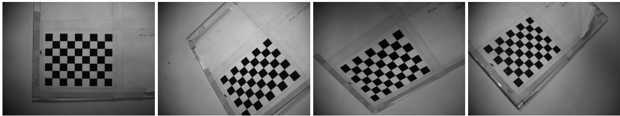
Figure 19: Four out of 11 checkerboard images used for camera and hand-eye calibration.
