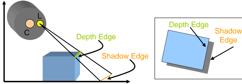
Figure 5: Depth and shadow edges. (Left) C denotes the camera and L denotes one of the light sources. Depth edges are attached to the object, while shadow edges are defined as the boundary between the shadow and the background. (Right) Depth and shadow edges in the camera image.
