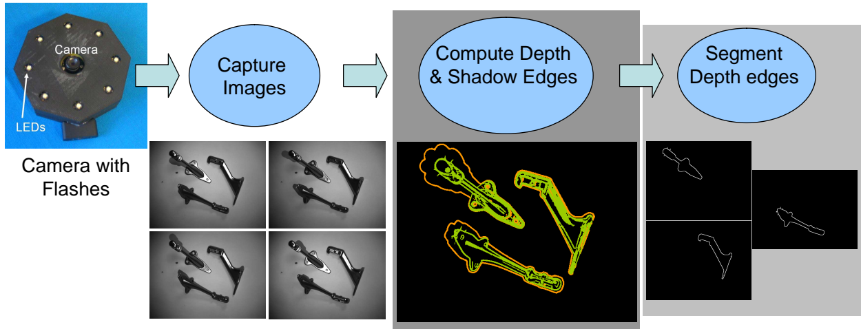
Figure 2: Flowchart of our approach. Eight images are captured by turning on LED’s surrounding the camera in succession (only four are shown for simplicity). Cast shadows are utilized to compute depth edges (green) and shadow edges (orange) in the scene. Depth edges are then segmented into silhouettes corresponding to different objects. Each silhouette is then used to estimate the 3D pose of the corresponding object as shown in Figure 3.
