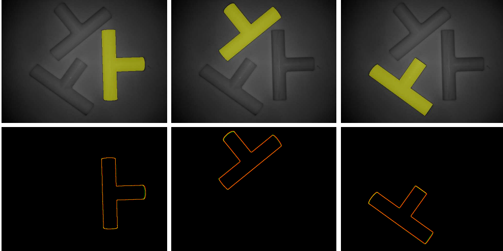
Figure 15: Pose estimation results on objects shown in Figure 14. Top row shows the overlay of the rendered CAD model on I_0 and the bottom row shows the overlay of the rendered CAD model silhouette on the segmented object silhouette according to the final estimated pose for all three objects.
