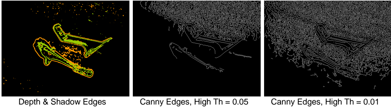
Figure 12: Non-uniform shiny background. Our technique results in reliable depth edges. In comparison, Canny intensity edges (on ambient illumination image) results in significant noise due to non-uniform illumination and metallic background. Shown are the Canny edge detection results using two different thresholds. Increasing the threshold reduces noise but also loses important edges of the objects.
