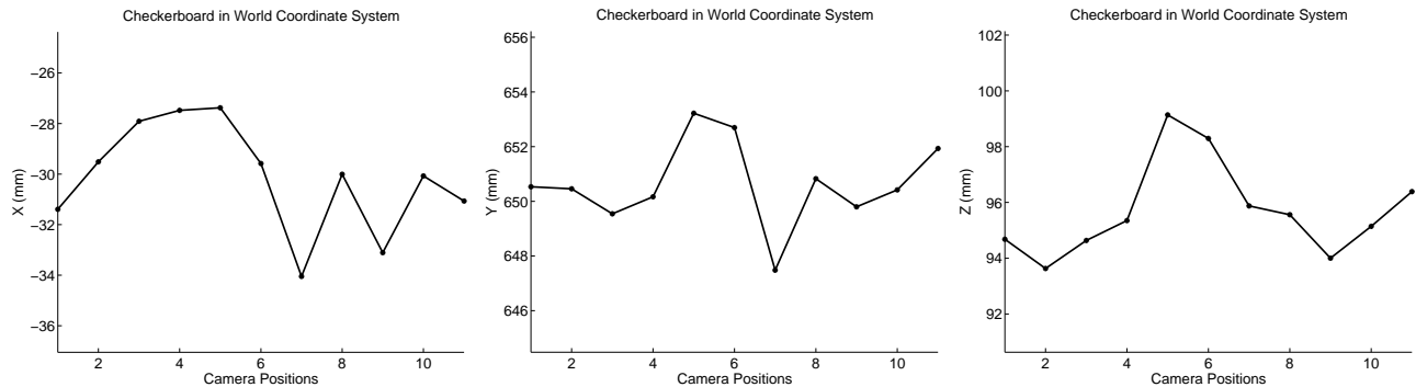
Figure 20: Location of one of the corners of the checkerboard in the world coordinate system for all 11 views.
