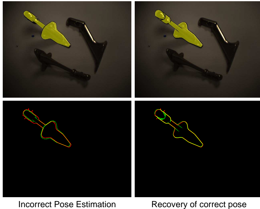
Figure 23: Ambiguities in pose estimation arise if the external silhouettes are similar for different poses as shown above. The coarse pose estimate followed by fine pose refinement results in an incorrect pose as shown on the left. The object is rotated along the pre-define axis by 180^\circ and fine pose refinement is performed again to check if it matches better, resulting in the correct pose.
