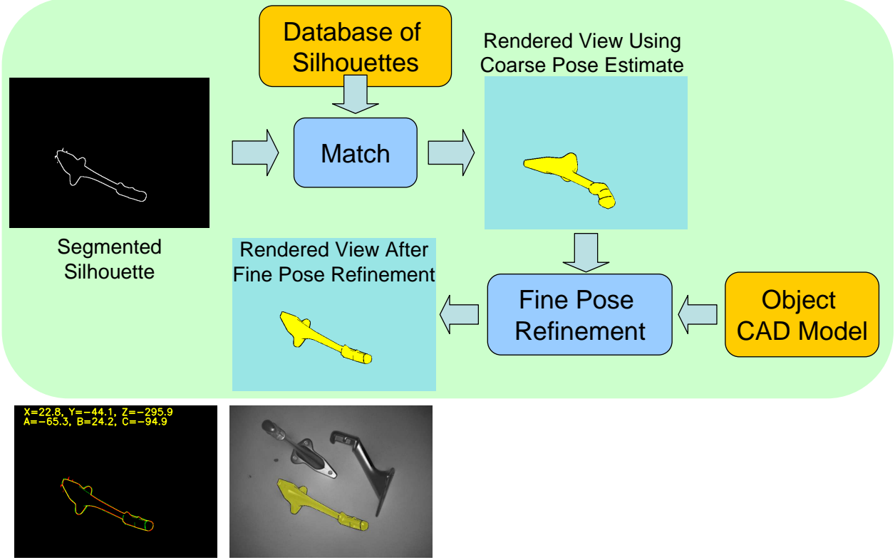
Figure 3: Flowchart describing 3D pose estimation. The pose for each object is estimated using the corresponding segmented silhouette. A coarse pose estimate is achieved by feature matching with a pre-computed database of silhouette features to obtain approximate rotation angles. Fine pose refinement using the CAD model is then performed to estimate accurate rotation and translation of the object. Overlay of the rendered CAD model on I_0 and the rendered CAD model silhouette on the segmented object silhouette using the final estimated pose is shown at the bottom for one of the object.
