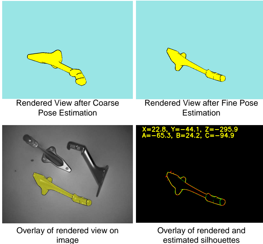
Figure 9: Pose estimation results on object 2. (Top Left) Rendered CAD model using rotation angles obtained after coarse pose estimation. (Top Right) Rendered CAD model after fine pose refinement, which updates all six rotation and translation parameters. (Bottom Left) Overlay of the rendered CAD model on I_0 according to the final estimated pose. (Bottom Right) Overlay of the rendered CAD model silhouette (green) on the segmented object silhouette (red) shows the success of the fine pose refinement. X, Y, Z denote translation and A, B, C denote rotation angles after fine pose refinement.
