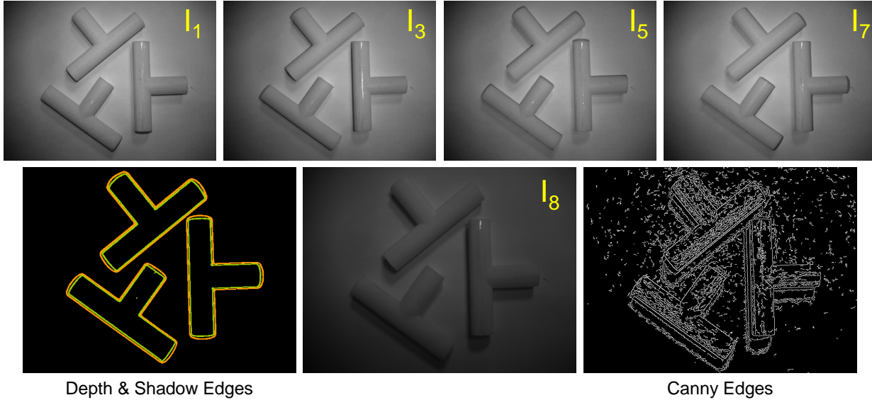
Figure 14: White objects on white background. Texture-less and colorless objects are difficult to handle for stereo based 3D reconstruction algorithms. Useful intensity edges are also not obtained on such scenes. In contrast, our technique works well on such scenes since depth edges are obtained by casting shadows. The extracted depth edges are significantly better compared to Canny edges on I_0 .
