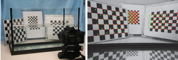
Figure 6. (Left) Setup. (Right) Photo captured by looking through a water tank. Projected 3D points are overlaid by applying pose estimated using CA (green) and our algorithm (red).
