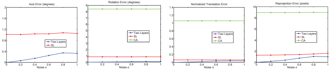
Figure 8. As noise increases, a two layer refraction system (Case 3) can be well-approximated using a single layer (SL) system (Case 1), but not using a central approximation.
