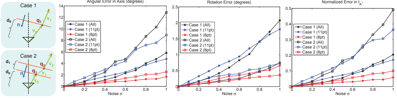
Figure 2. (Left) Single layer (Case 1) and two layer (Case 2, \mu_2 = \mu_0 ) configurations. (Right) Comparison of 11pt and 8pt algorithm for estimation of axis, rotation and t_{A^\perp} using coplanarity constraints.
