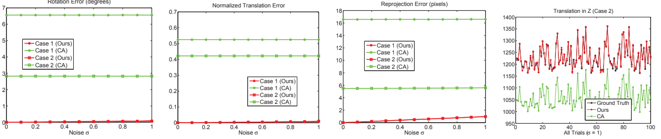
Figure 3. Comparison of rotation, translation and reprojection error using our algorithm with a central approximation (CA) for Case 1 and Case 2. The right most plot shows the estimated t_z for Case 2 over all 100 trials for \sigma = 1 pixel. CA estimates the object to be closer to the camera.
