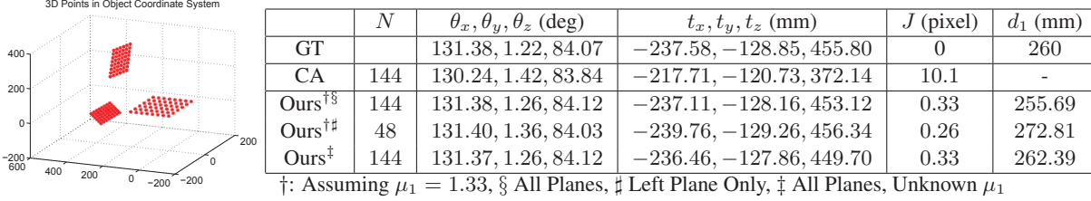
Figure 5. (Left) 3D points in the left checkerboard coordinate system. (Right) Estimates of pose and water-tank thickness d_1 , and the final reprojection error J for real data shown in Figure 6 using central approximation (CA) and our algorithm. GT denotes ground-truth and N denotes the number of 2D-3D correspondences used.
