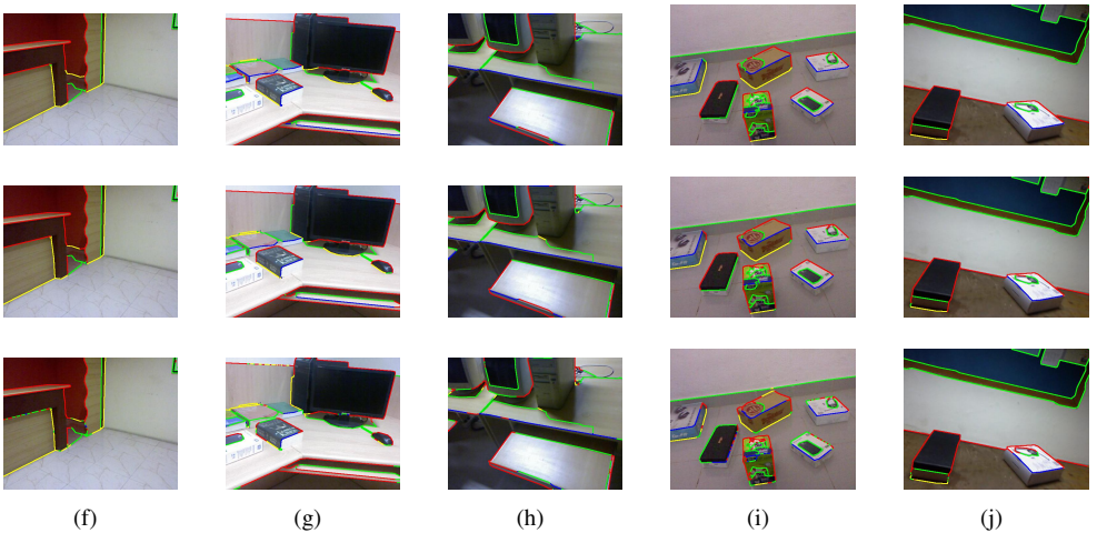
Figure 6: Ground truths (above) and the corresponding results from our approach (2 nd row) and Gupta et al. [6] (3 rd row). Color code: red (occ), green (pln), blue (cvx), yellow (ccv).
