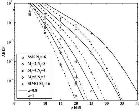
Fig. 9. The performance of FD-TWRC-SM for various sizes of signal and spatial constellation diagrams at 4bpcu data rate. Markers show Monte Carlo simulations based on 10^6 realizations, and solid lines and dashed lines show the analytical union-bounds.
