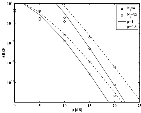
Fig. 10. The performance of FD-TWRC-SM for various sizes of spatial constellation diagrams at BPSK signal constellation diagram. Markers show Monte Carlo simulations based on 10^6 realizations, and solid lines and dashed lines show the analytical union-bounds.
