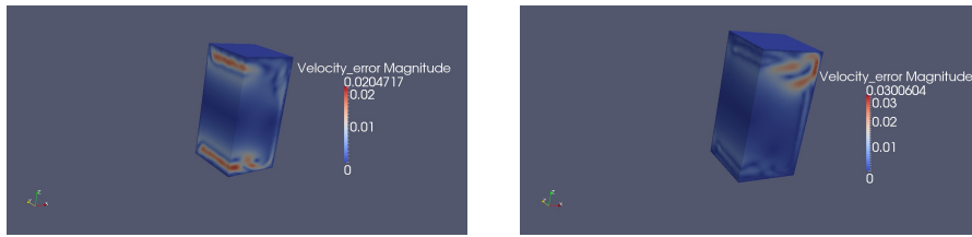
Figure 3: ROM-G velocity errors profile (right-side: ROM-G, left-side: ROM-G-Learning)- Case one
