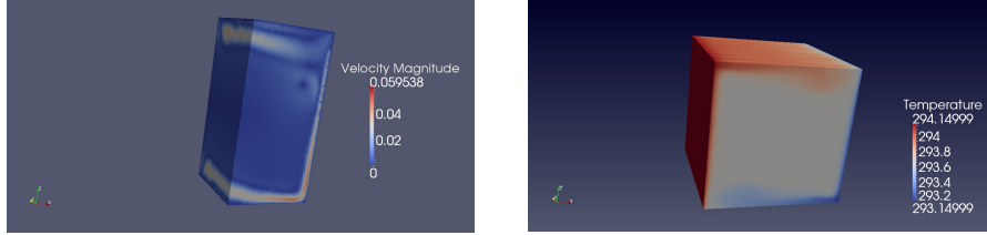
Figure 1: True solution profile (right-side: velocity, left-side: temperature)-Case one
