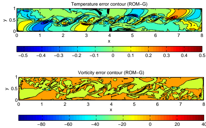
Figure 19: ROM-G-Learning error profile snapshot at 8[sec] (top: temperature, bottom: vorticity)- Case three
