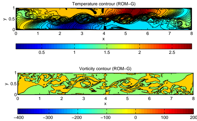
Figure 18: ROM-G-Learning solution profile snapshot at 8[sec] (top: temperature, bottom: vorticity)- Case three
