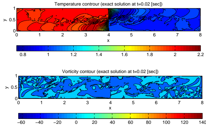
Figure 13: True solution profile snapshot at 0.02[sec] (top: temperature, bottom: vorticity)- Case three
