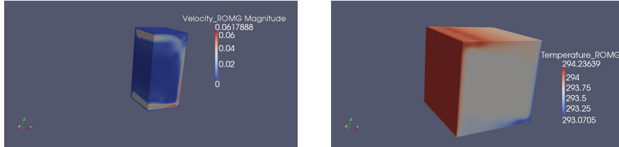
Figure 5: ROM-G-Learning solution profile (right-side: velocity, left-side: temperature)- Case one
