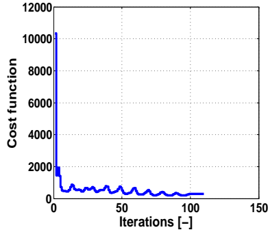
Figure 17: Learning cost function vs. number of learning iterations- Case three
