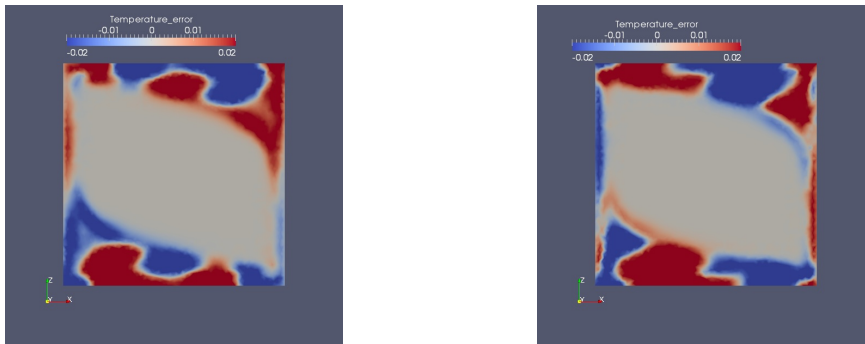
Figure 4: ROM-G temperature errors profile (right-side: ROM-G, left-side: ROM-G-Learning)- Case one
