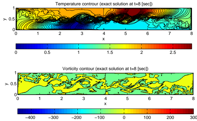
Figure 14: True solution profile snapshot at 8[sec] (top: temperature, bottom: vorticity)- Case three
