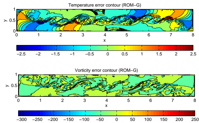
Figure 16: POD-ROM-G (no closure) error profile snapshot at 8[sec] (top: temperature, bottom: vorticity)- Case three
