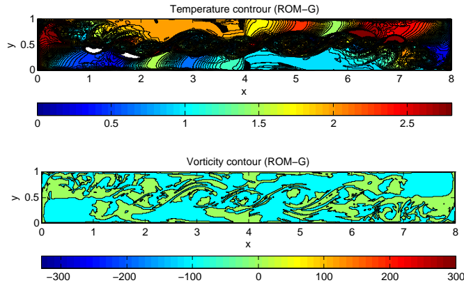
Figure 15: POD-ROM-G (no closure) solution profile snapshot at 8[sec] (top: temperature, bottom: vorticity)- Case three
