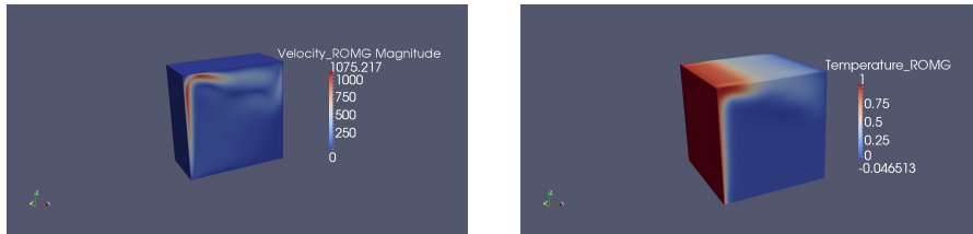
Figure 10: ROM-G-Learning solution profile (right-side: velocity, left-side: temperature)- Case two
