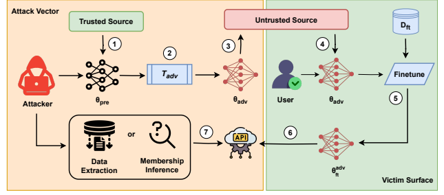
Figure 1: Overview of the threat model and steps of the attack: (1) Attacker downloads a pre-trained LLM, (2) Poisons the model with an algorithm, T_{adv} , and (3) release the model. (4) The victim downloads the poisoned LLM, (5) fine-tunes on their private data, and (6) releases the API-based query access to the model. (7) Finally, the adversary conducts membership inference or data extraction.
